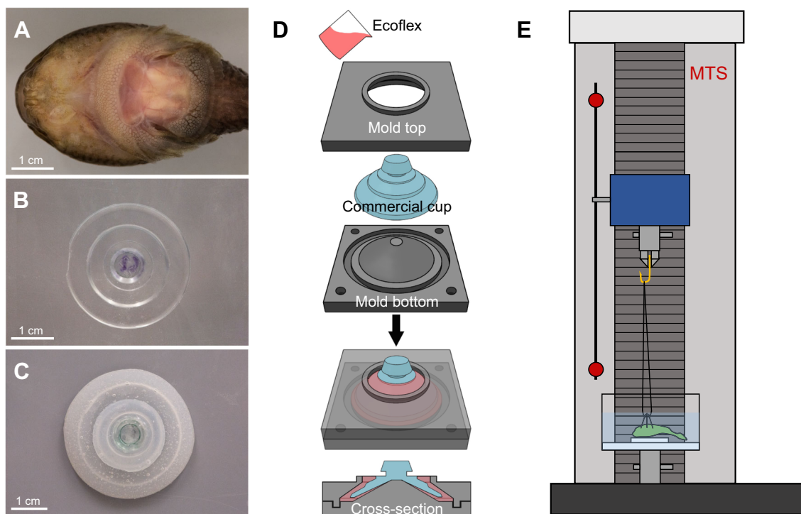
Fig. 1. Suction cups and the experimental setup used measure their adhesive forces. (A–C) Examples of the three types of cups tested in this study: (A) the northern clingfish, (B) a commercial suction cup and (C) an overmolded commercial cup. (D) Schematic representing the overmolding procedure used to add a silicone disc rim to the commercial cups. (E) Our test setup to measure the pull-off forces of each cup, including the harness used to attach the clingfish to the moving crosshead of the MTS materials testing machine (drawing from Huie and Summers, 2022).
